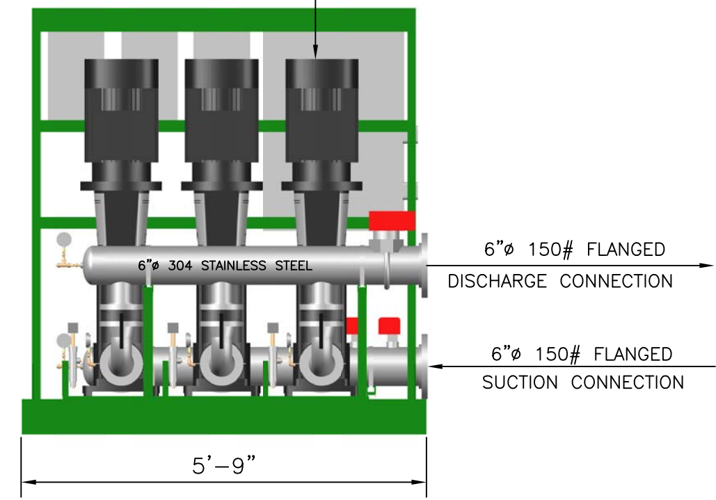
(3) GRUNDFOS CRN45-2-2 PUMPS 15 H.P. @ 3500 RPM TEFC/PE MOTORS 460/3/60 Hz.
