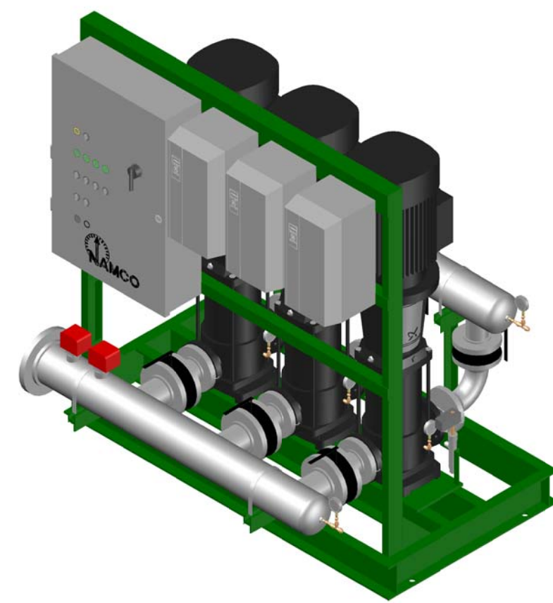
(3) GRUNDFOS CRN45-2-2 PUMPS 15 H.P. @ 3500 RPM TEFC/PE MOTORS 460/3/60 Hz.
